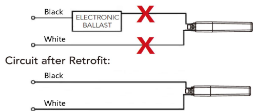
Wiring Diagram for Electronic Ballast
